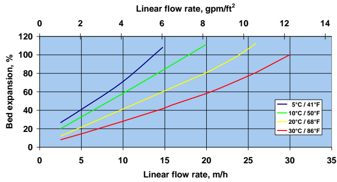
Figure 19 Backwash expansion
