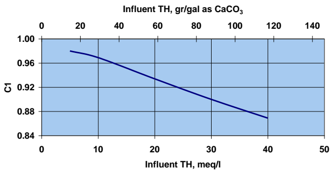
Figure 11 C1 - Capacity correction factor for Total Hardness
