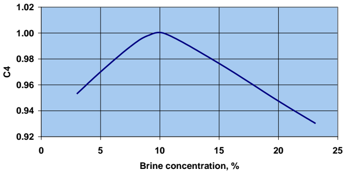
Figure 5 C4 - Capacity correction factor for brine concentration
