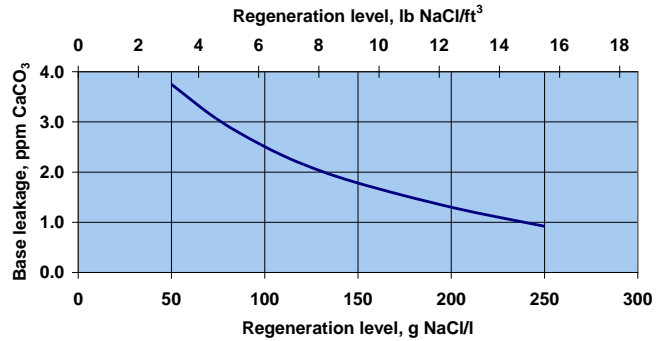
Figure 6 Base hardness leakage
