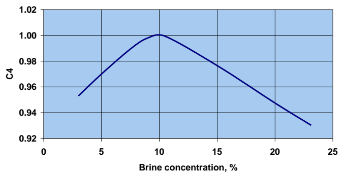
Figure 14 C4 - Capacity correction factor for brine concentration
