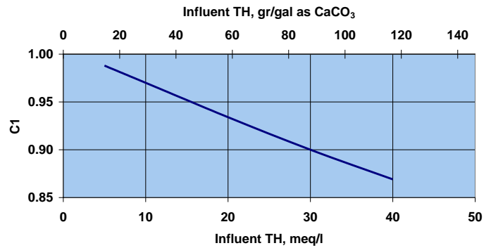
Figure 2 C1 - Capacity correction factor for influent TH
