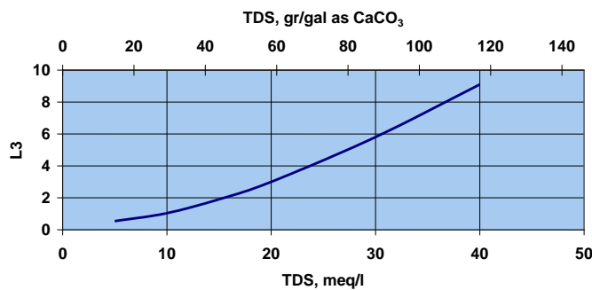
Figure 9 L3 - Leakage correction factor for Total Dissolved Solids
