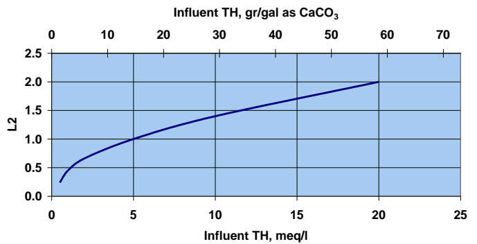
Figure 8 L2 - Leakage correction factor for Total Hardness
