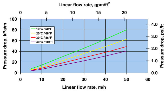
Figure 20 Pressure drop
