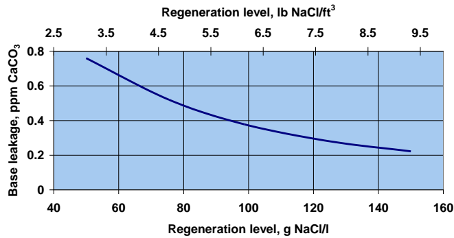
Figure 15 Base hardness leakage
