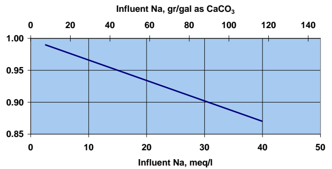
Figure 4 C3 - Capacity correction factor for influent Na
