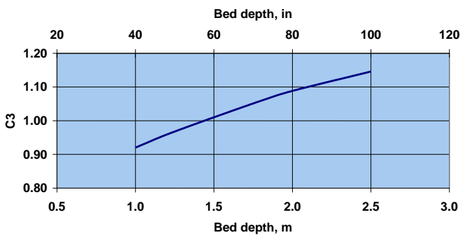
Figure 13 C3 - Capacity correction factor for resin bed depth
