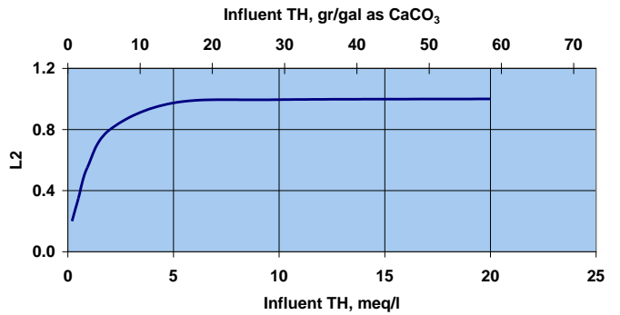
Figure 17 L2 - Leakage correction factor for Total Hardness
